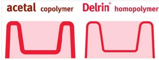
Figure 12: The superior mechanical properties of Delrin ® homopolymer can allow thinner wall sections compared to acetal copolymers for the same physical part capabilities.
